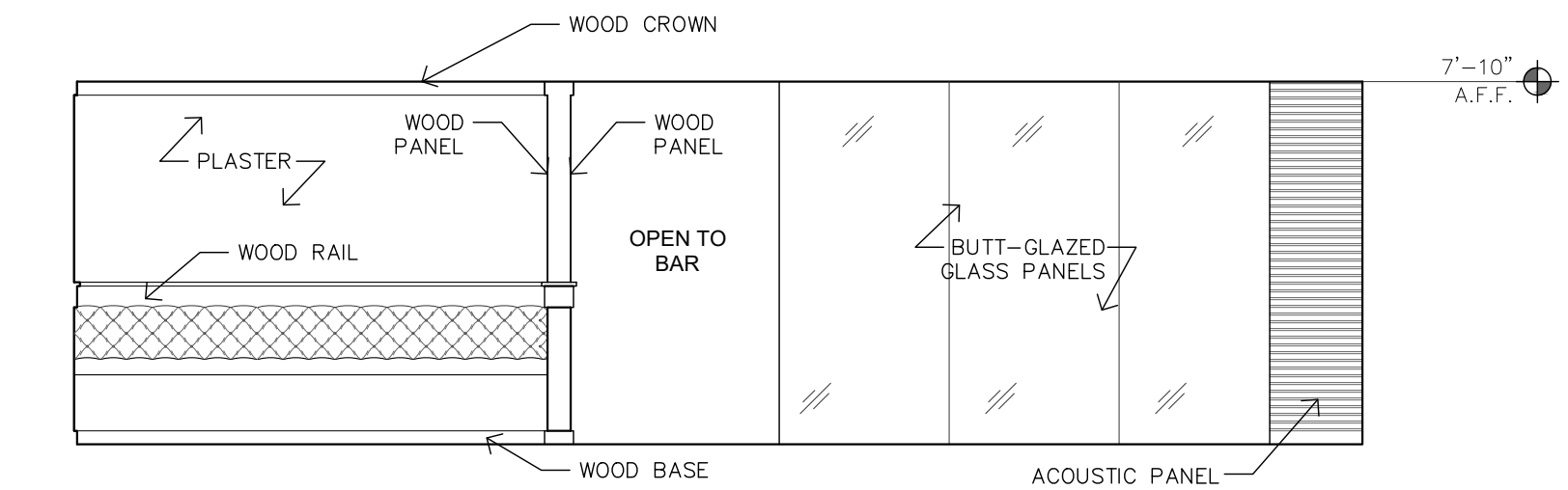
11 ENTRY - SOUTH 1/4" = 1'-0"
