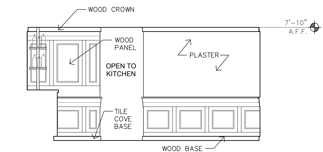
08 BAR - SOUTH 1/4" = 1'-0"
