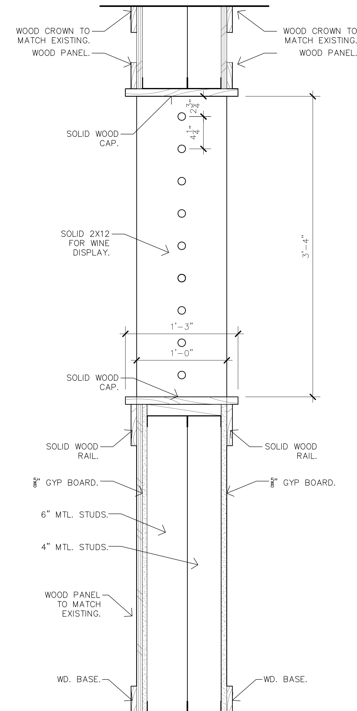
02 SECT. @ PARTITION 1-1/2" = 1'-0"
