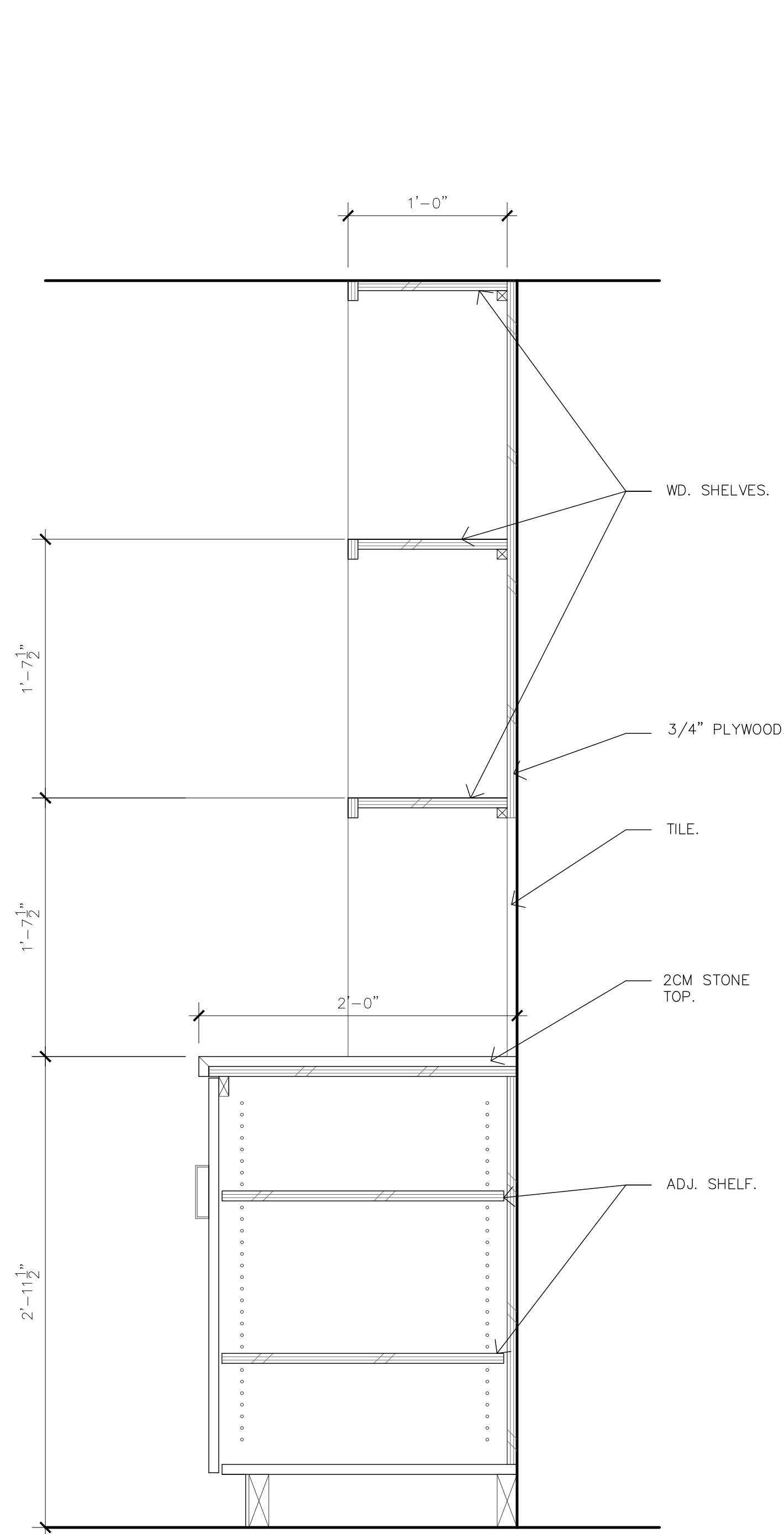
09 SECT. @ DINING I WAIT STATION 1-1/2" = 1'-0"
