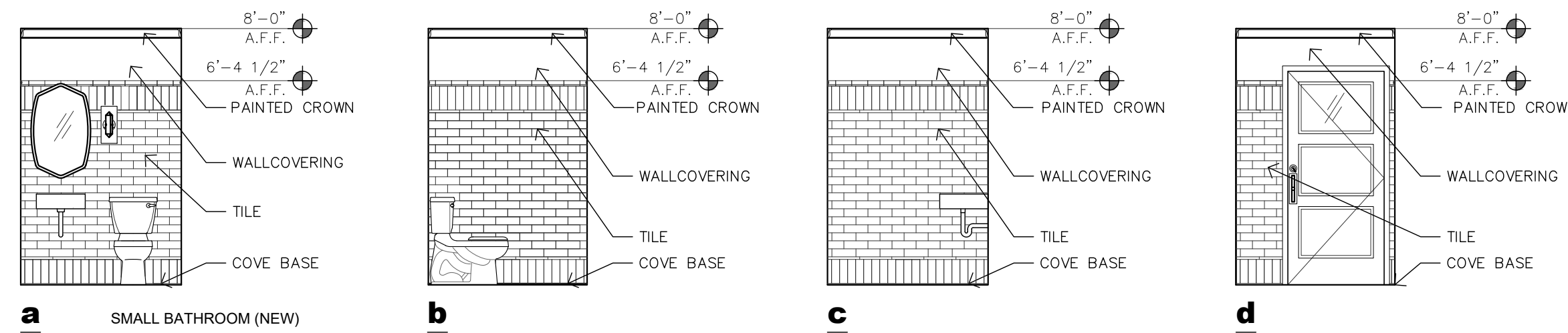
12 RESTROOM 1/4" = 1'-0"
