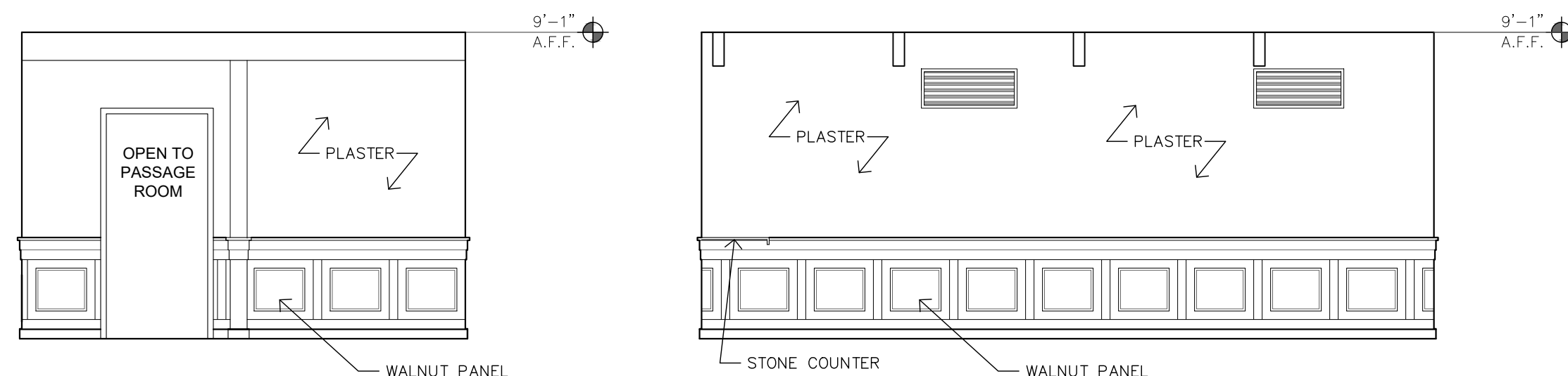
04 PRIVATE DINING - NORTH 1/4" = 1'-0"
