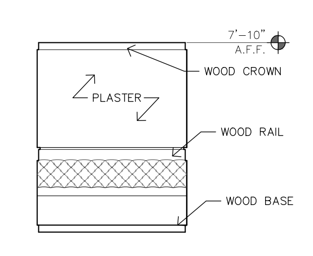
12 ENTRY - EAST 1/4" = 1'-0"
