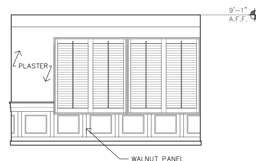
02 PRIVATE DINING - SOUTH 1/4" = 1'-0"
