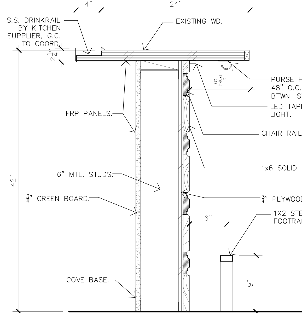
06 SECT. @ BAR COUNTER 1-1/2" = 1'-0"
