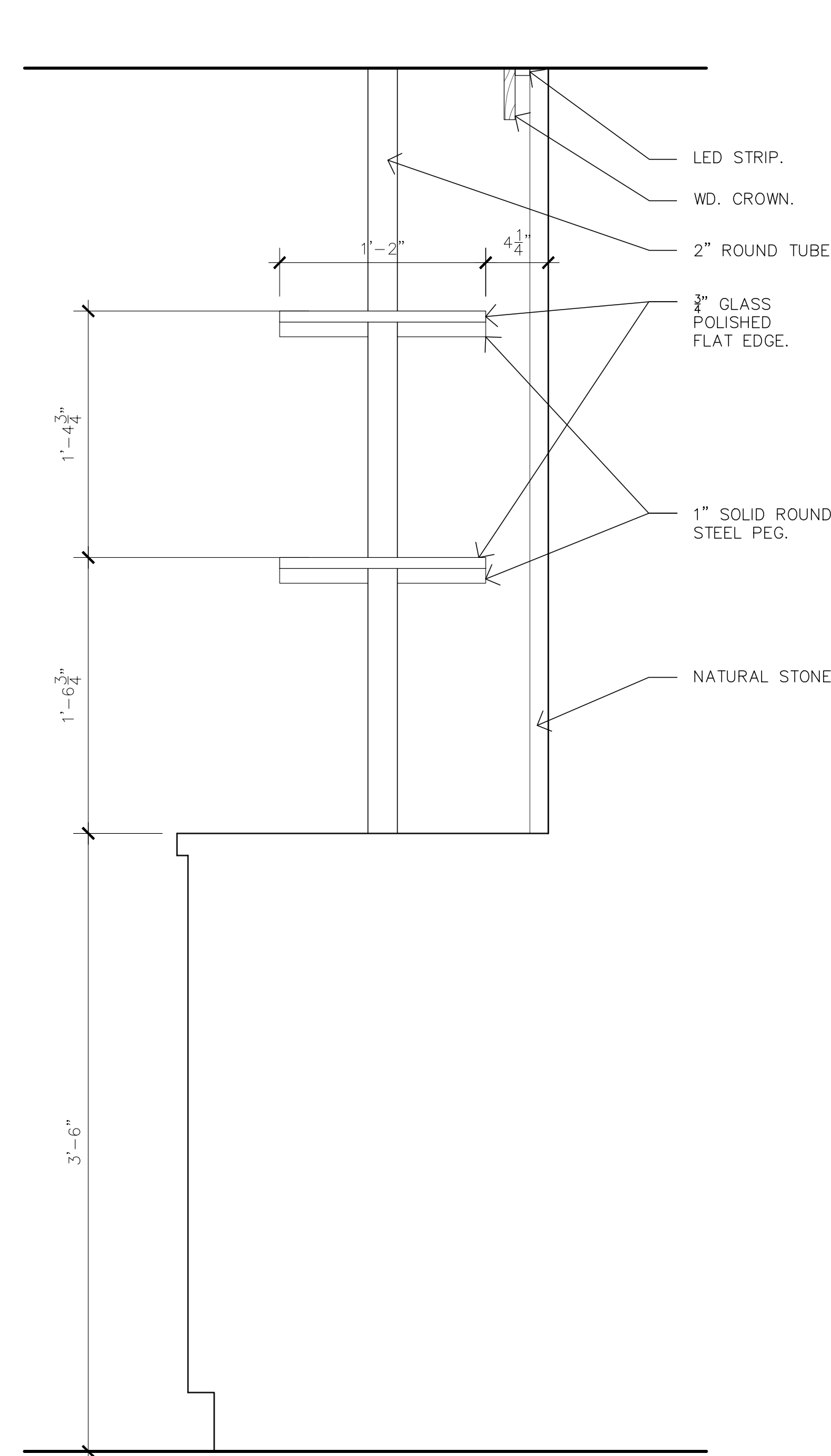
04 SECT. @ BACK BAR 1-1/2" = 1'-0"
