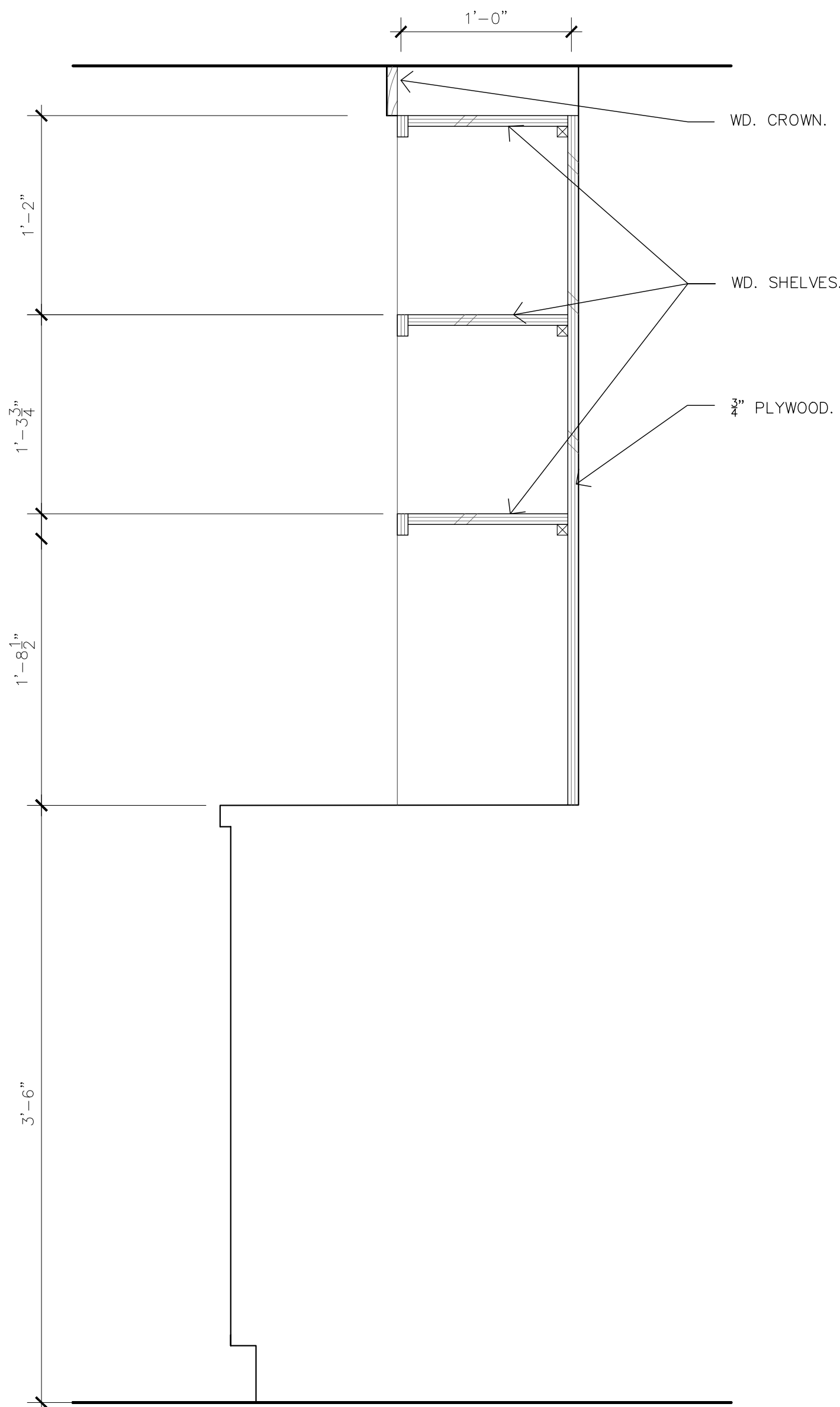
03 SECT. @ BAR WAIT STATION 1-1/2" = 1'-0"
