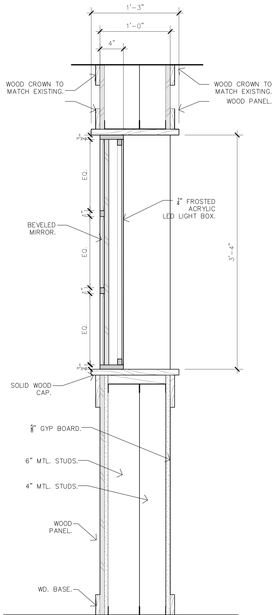
01 SECT. @ PARTITION W/ LIGHT BOX 1-1/2" = 1'-0"
