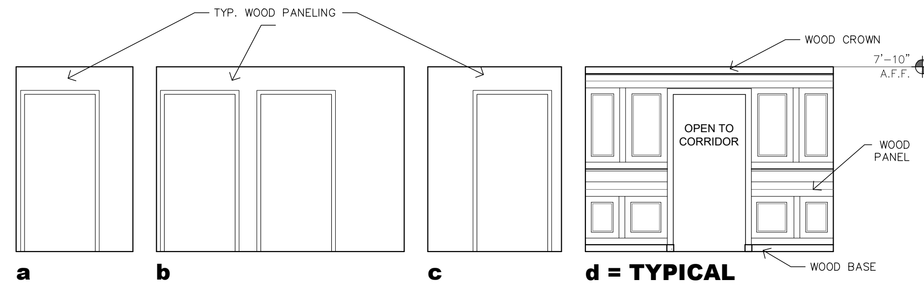
13 RESTROOM - VESTIBULE 1/4" = 1'-0"
