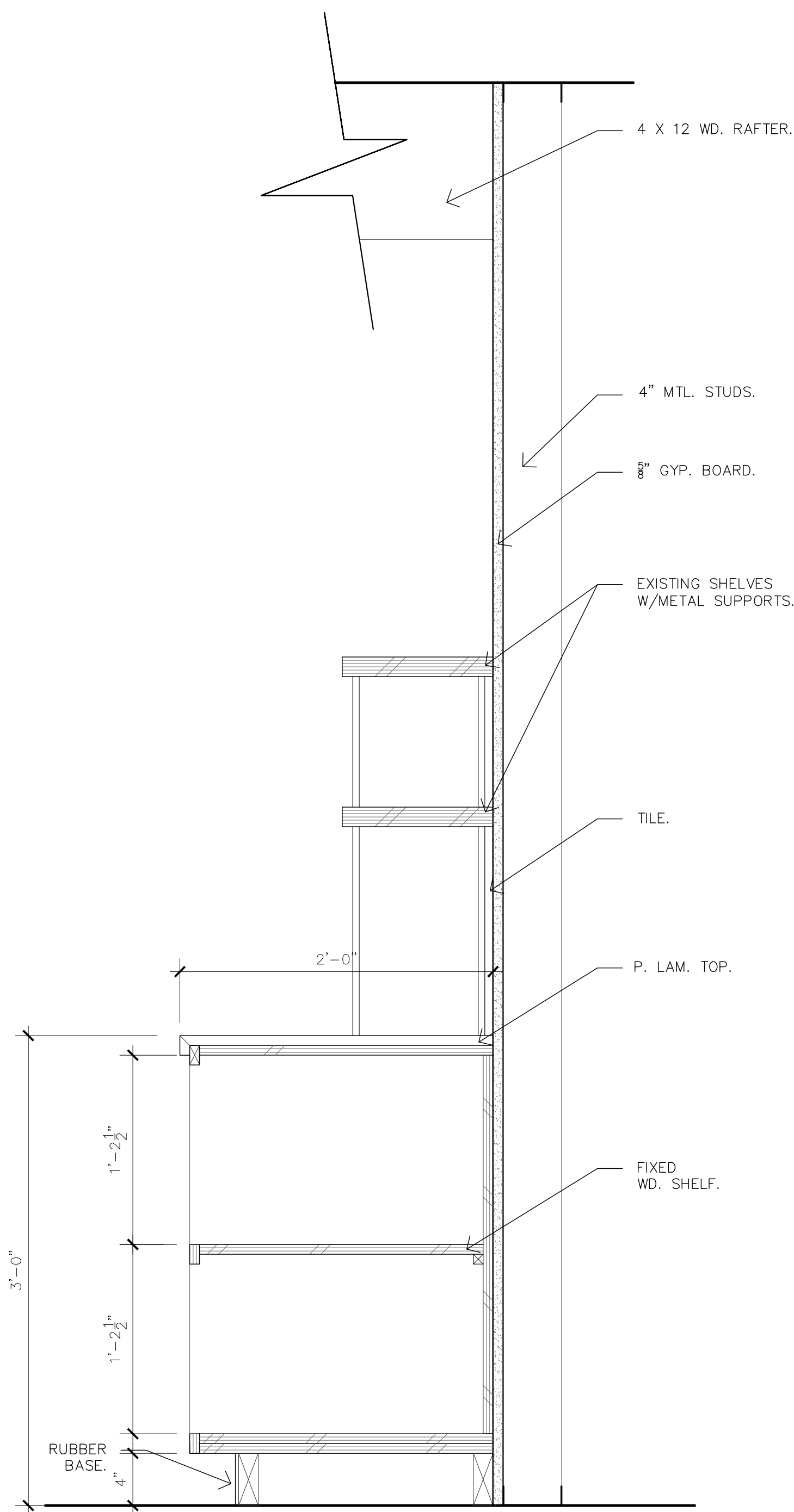
11 SECT. @ PASSAGE ROOM WEST 1-1/2" = 1'-0"
