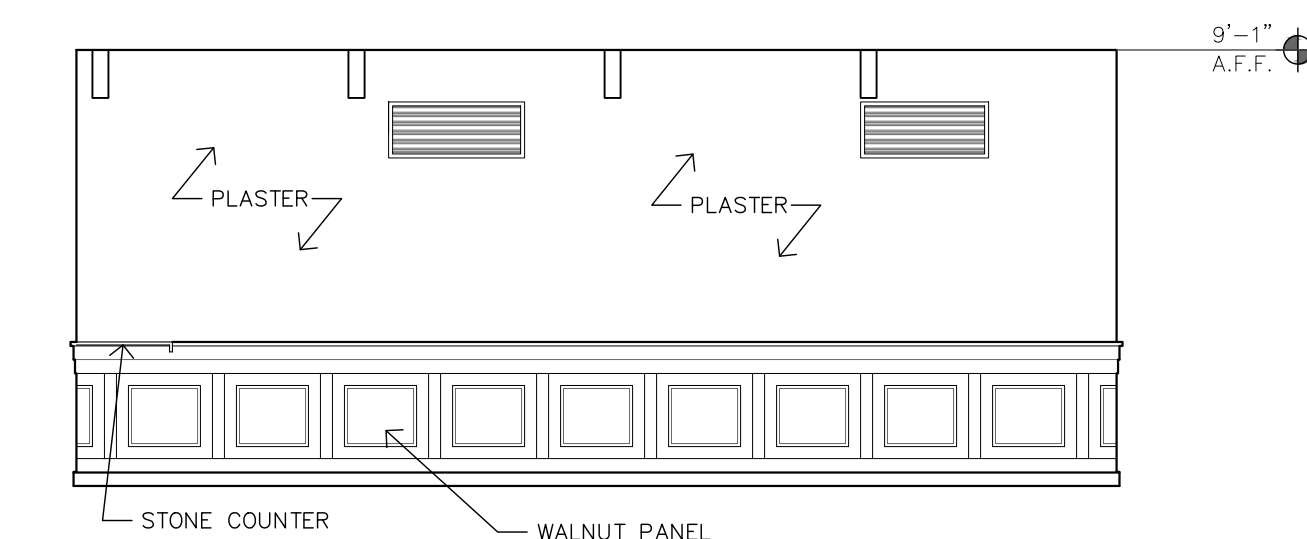
03 PRIVATE DINING - EAST 1/4" = 1'-0"
