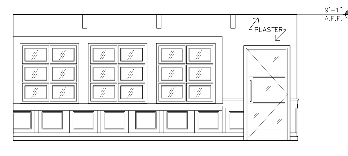
01 PRIVATE DINING - WEST 1/4" = 1'-0"
