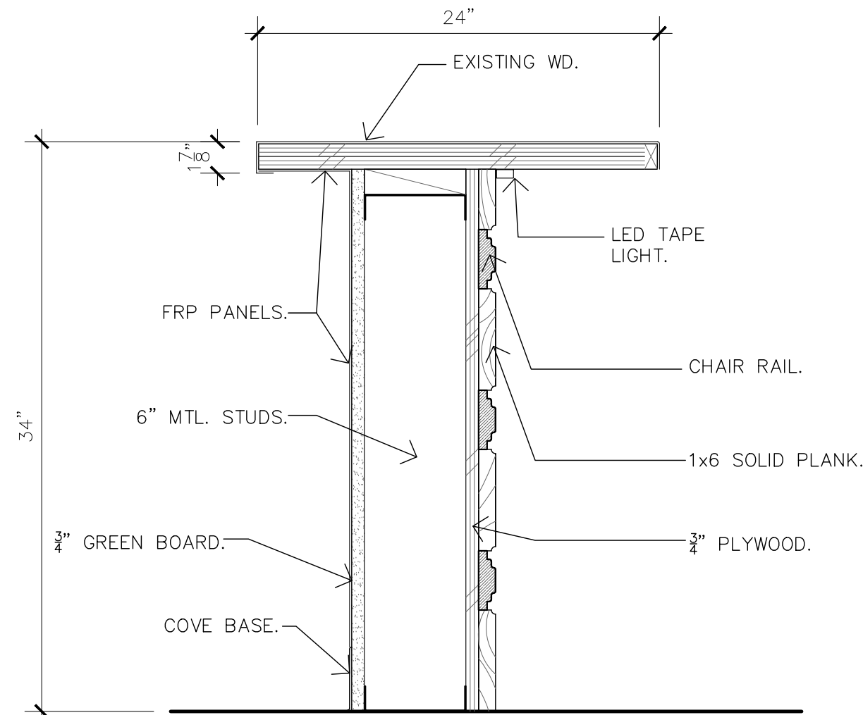
07 SECT. @ ADA COUNTER 1-1/2" = 1'-0"
