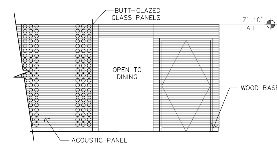
15 ENTRY - WEST 1/4" = 1'-0"
