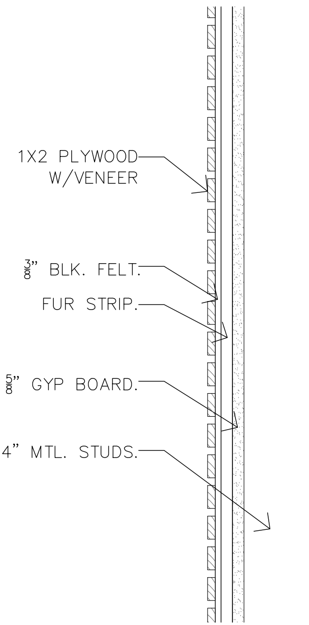
08 SECT. @ ACOUNSTIC PANEL 1-1/2" = 1'-0"
