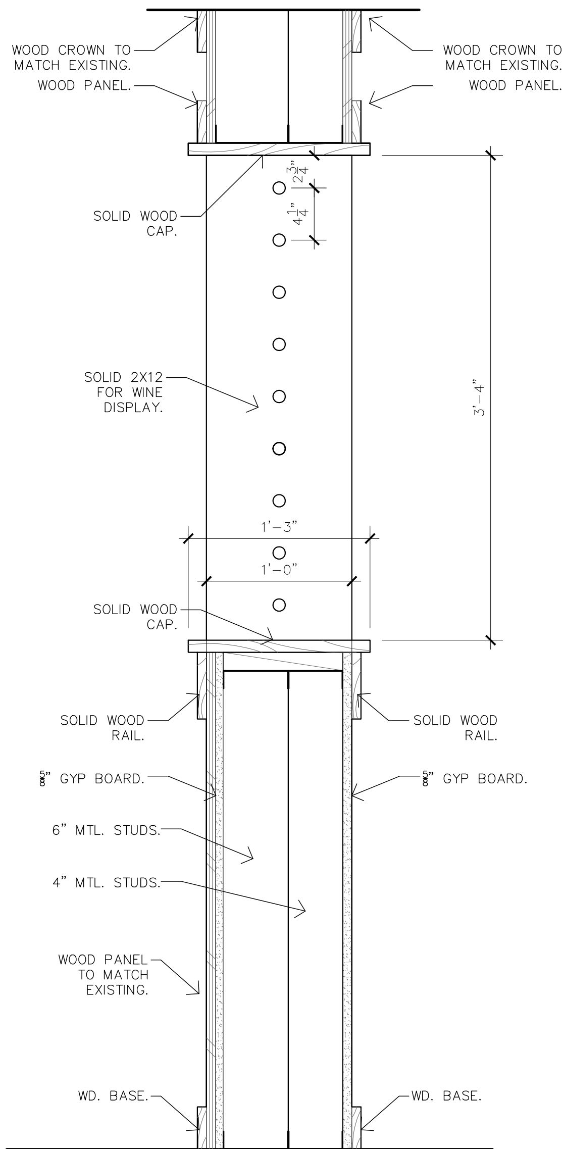
02 SECT. @ PARTITION 1-1/2" = 1'-0"
