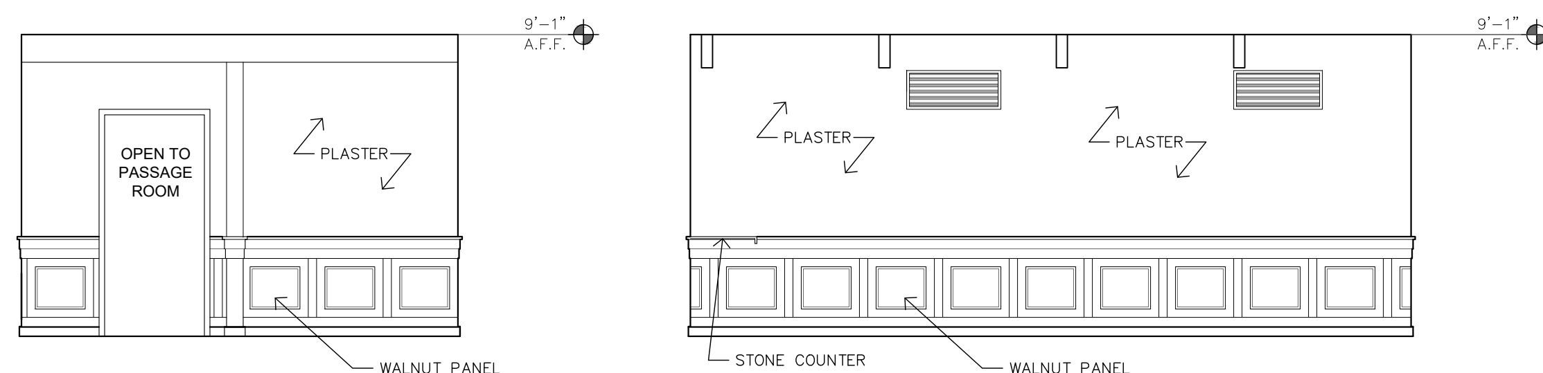
04 PRIVATE DINING - NORTH 1/4" = 1'-0"
