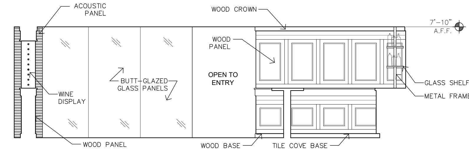
10 BAR - NORTH 1/4" = 1'-0"
