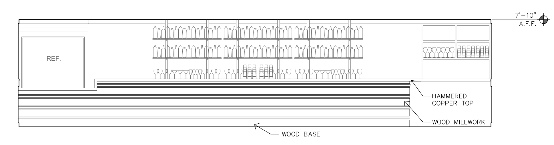
05 BAR - EAST 1/4" = 1'-0"
