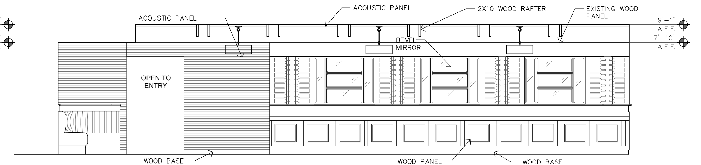
03 DINING - EAST 1/4" = 1'-0"
