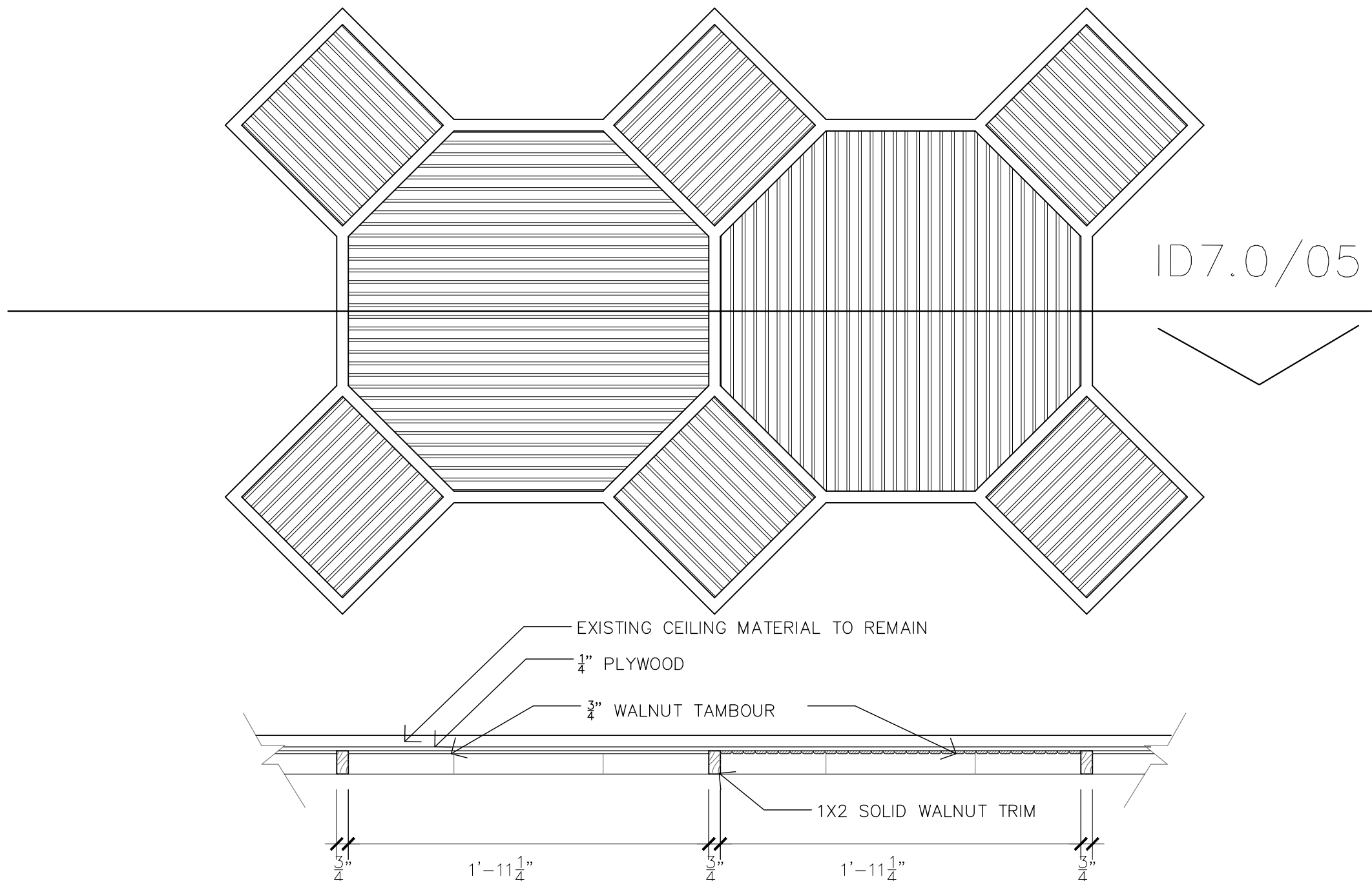
05 SECT. @ ENTRY / BAR CEILING 1-1/2" = 1'-0"
