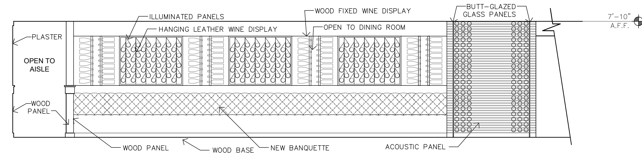
06 BAR - WEST 1/4" = 1'-0"
