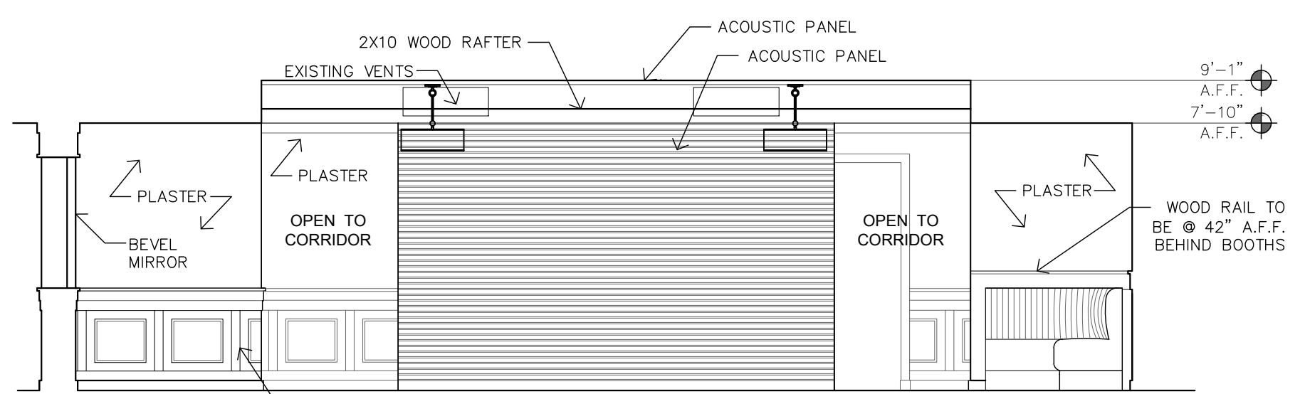
02 DINING - SOUTH 1/4" = 1'-0"
