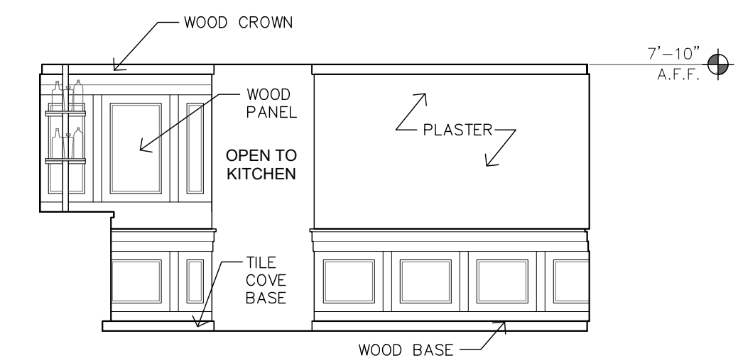
08 BAR - SOUTH 1/4" = 1'-0"
