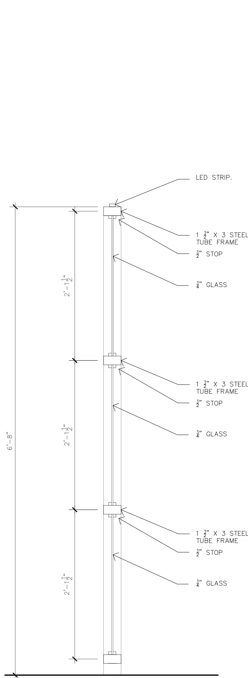
10 SECT. @ STEEL & GLASS PARTITION 1-1/2" = 1'-0"
