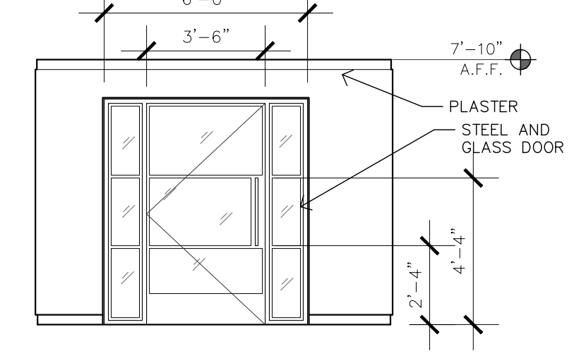
13 ENTRY - ENTRY DOOR 1/4" = 1'-0"
