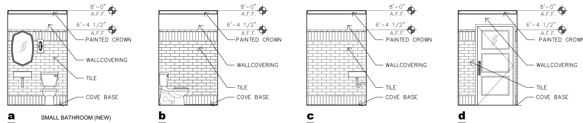
12 RESTROOM 1/4" = 1'-0"
