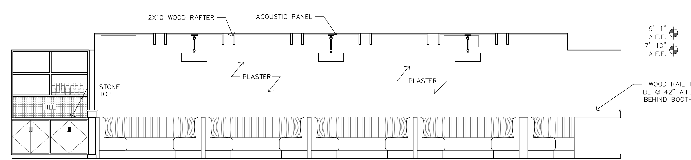
01 DINING - WEST 1/4" = 1'-0"
