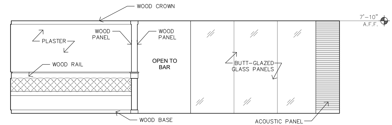
11 ENTRY - SOUTH 1/4" = 1'-0"
