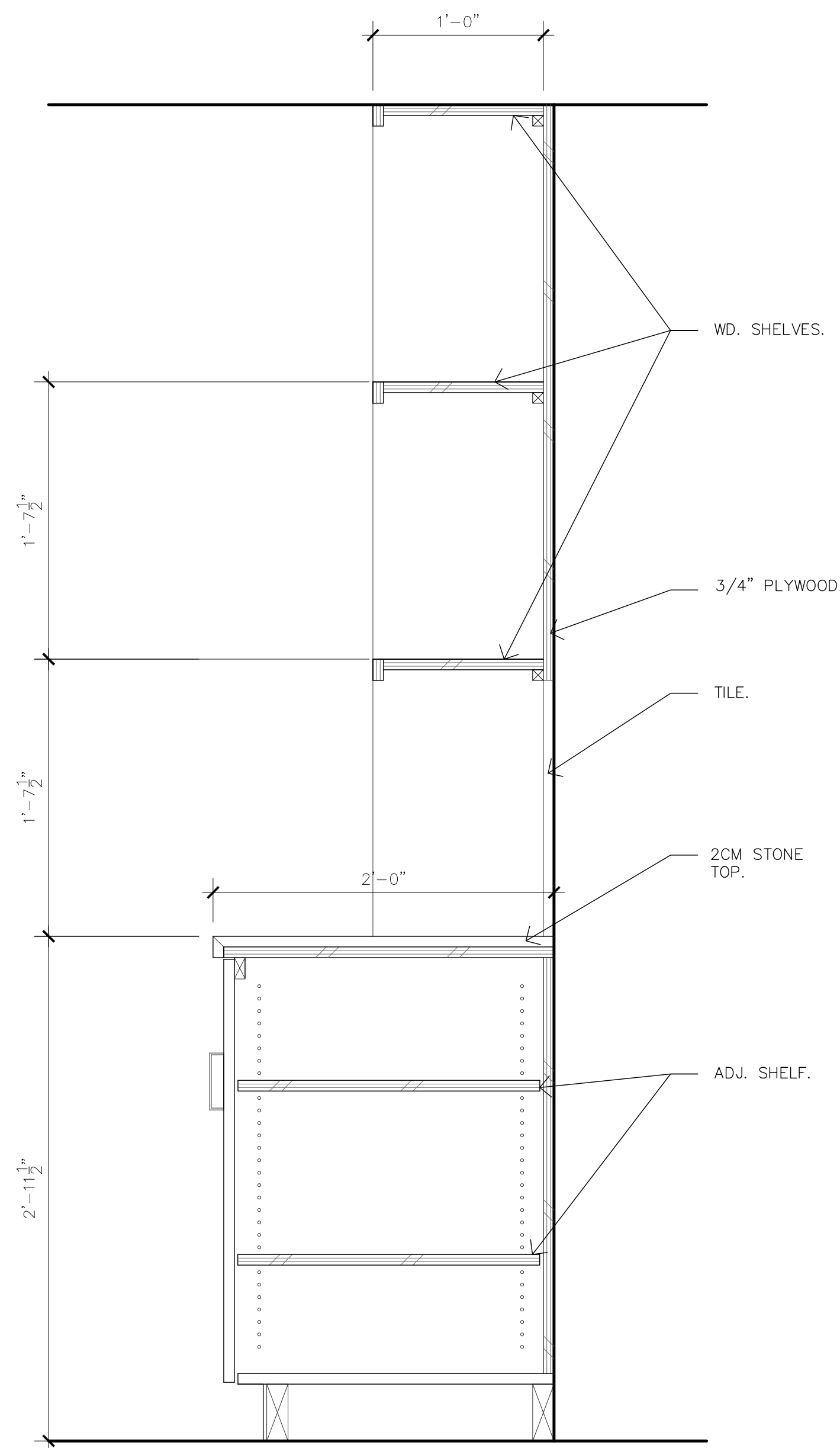
09 SECT. @ DINING I WAIT STATION 1-1/2" = 1'-0"
