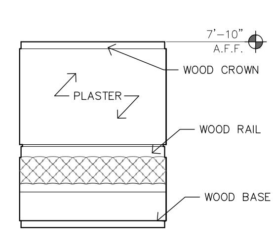
12 ENTRY - EAST 1/4" = 1'-0"
