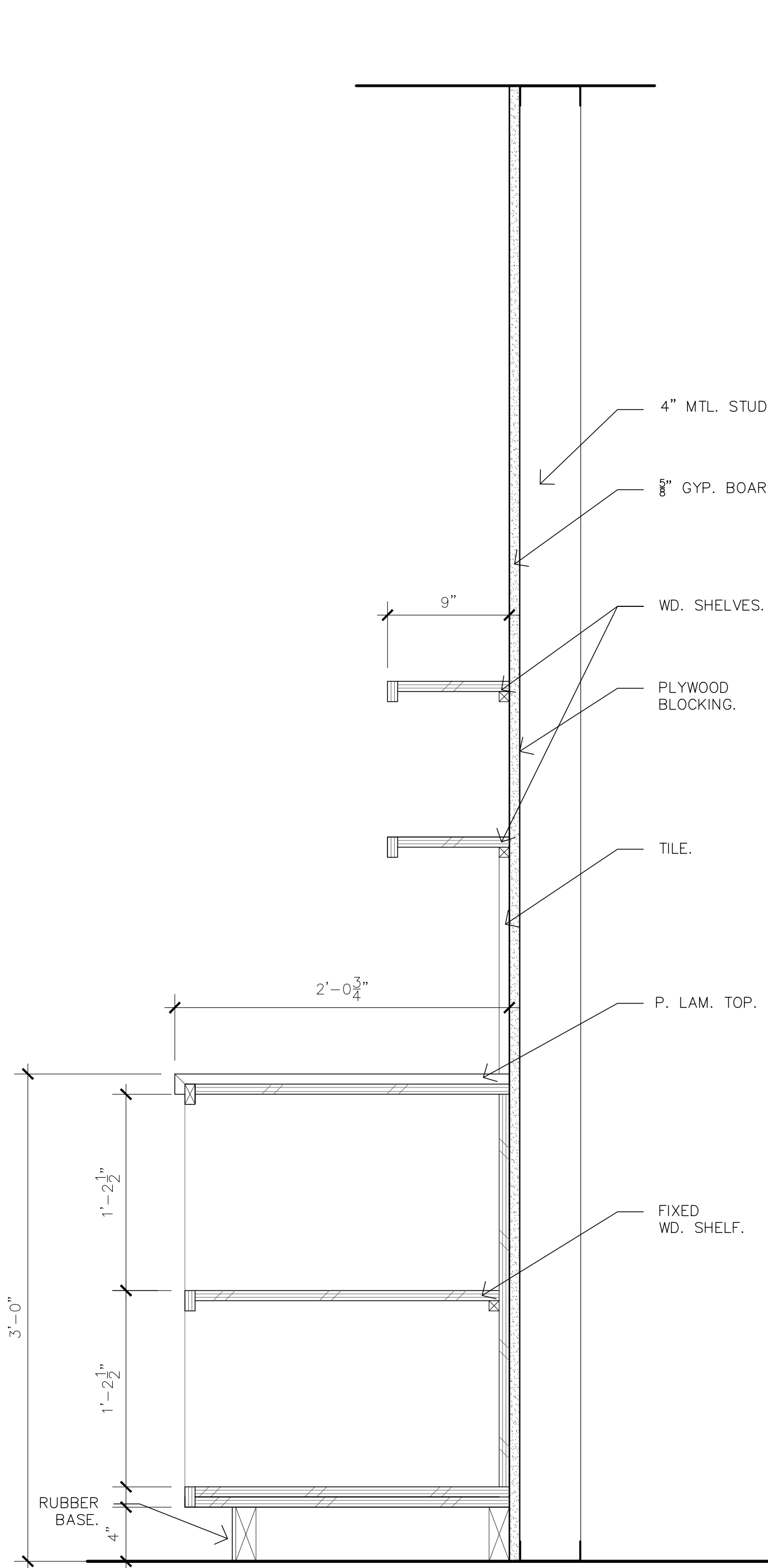
12 SECT. @ PASSAGE ROOM EAST 1-1/2" = 1'-0"
