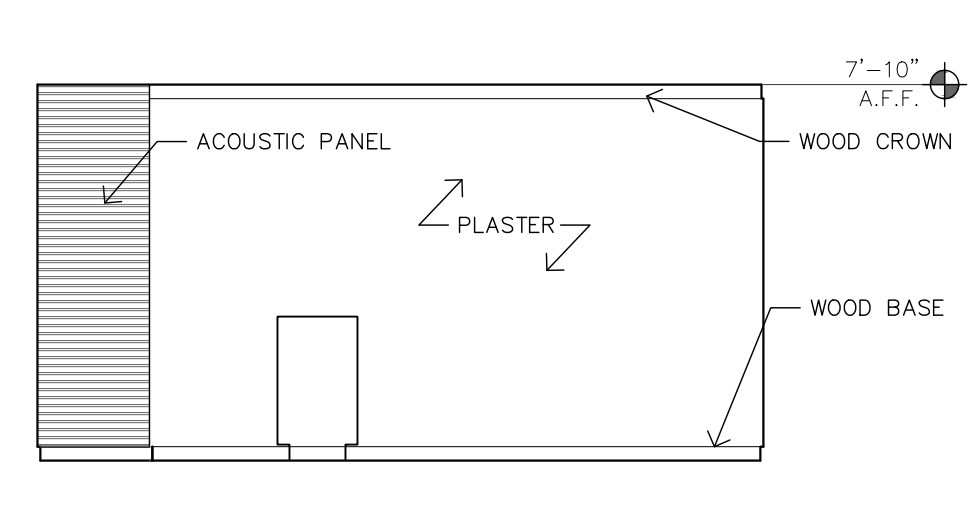
14 ENTRY - NORTH 1/4" = 1'-0"
