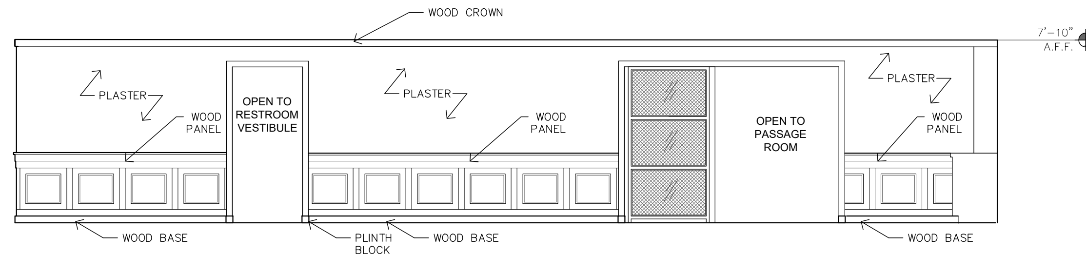
14 CORRIDOR - SOUTH 1/4" = 1'-0"
