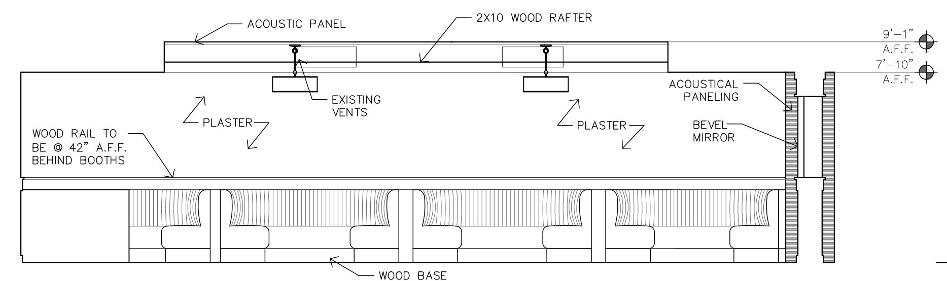
04 DINING - NORTH 1/4" = 1'-0"
